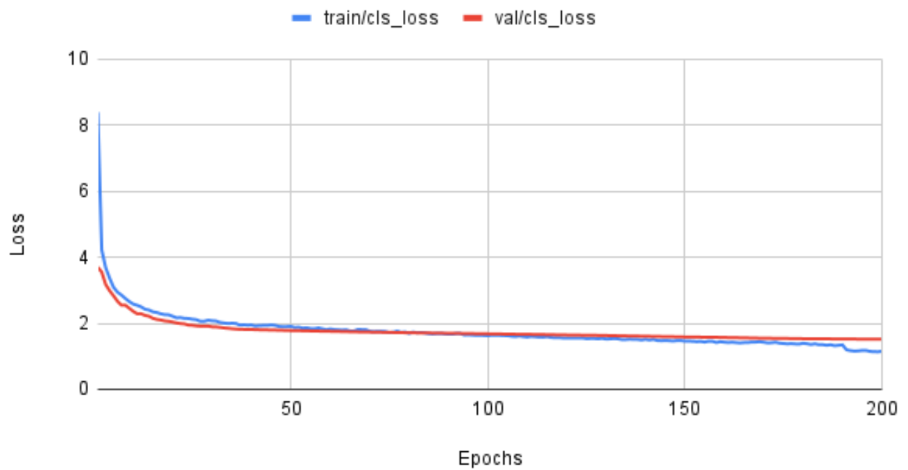
Fig. 17: Classification loss on the Baseline model. The blue line indicates the training loss and the red line indicates the loss of the validation data.
