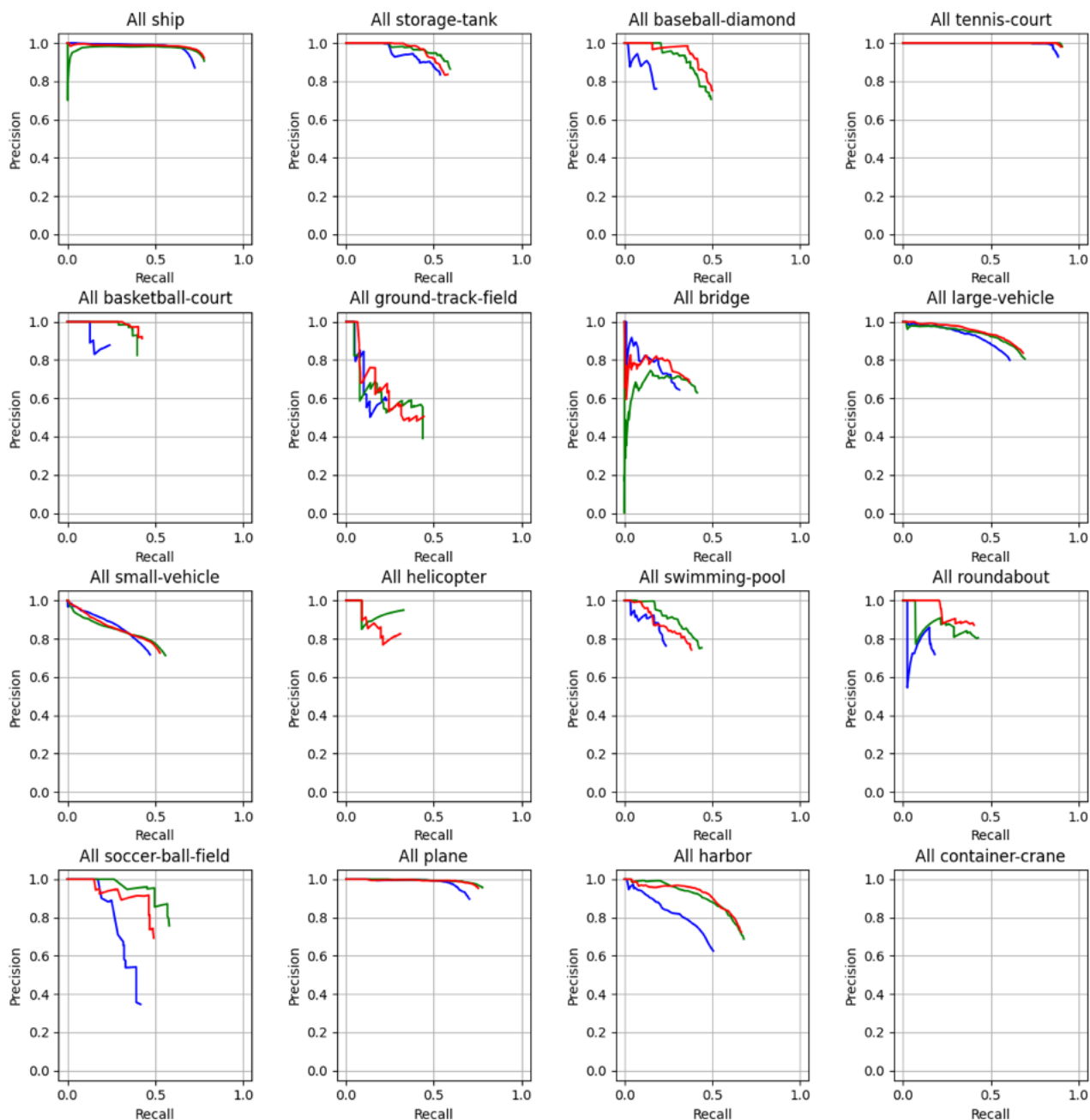
Fig. 7: Precision-Recall Curves for all instances. The blue line indicates the BL model, the green line the model from experiment 1 and the red line the model from experiment 2. Looking at all instances some classes benefit only from oversampling while other also benefit from the augmentation of the oversampled images.
