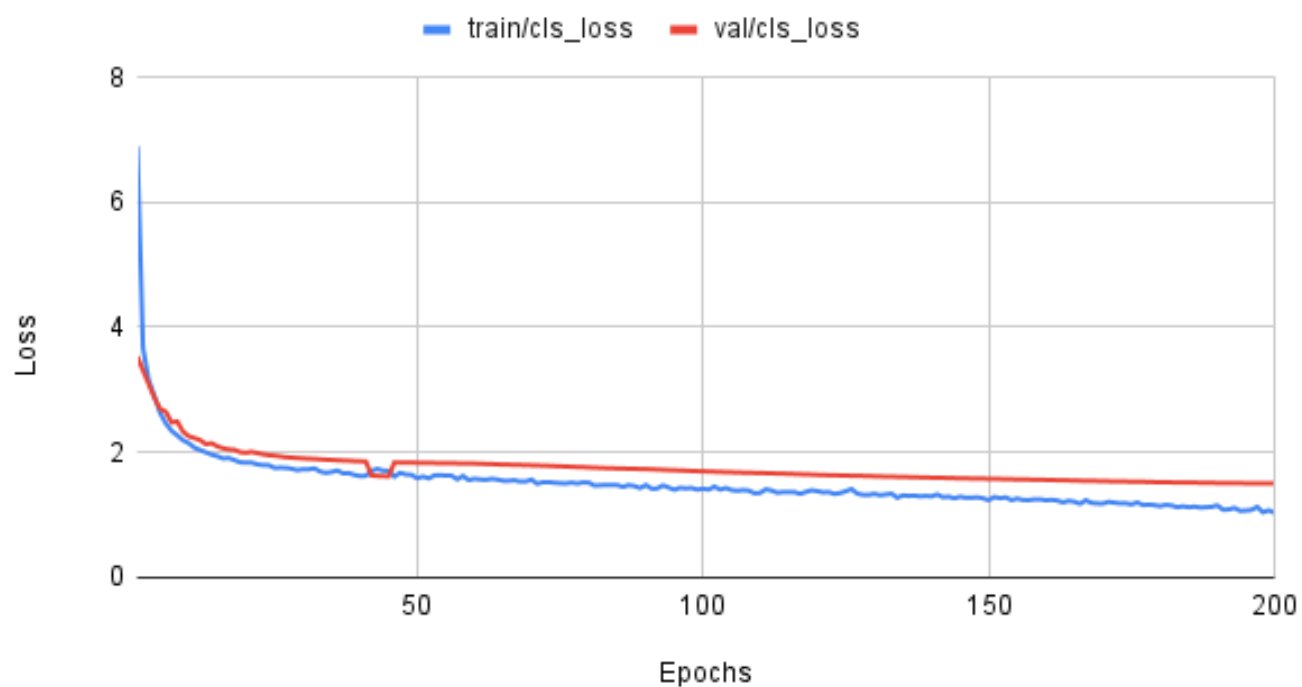
Fig. 23: Classification Loss on the Experiment 2 model. The blue line indicates the training loss and the red line indicates the loss of the validation data.
