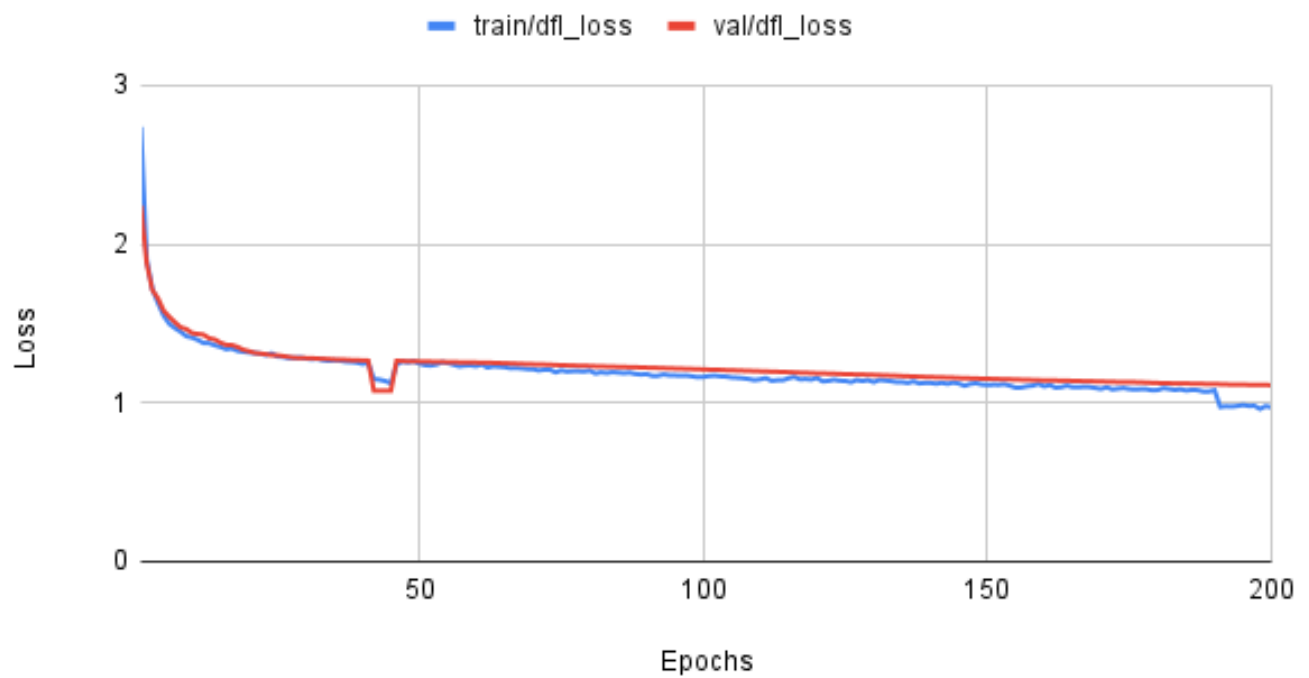
Fig. 24: Distribution Focal Loss on the Experiment 2 model. The blue line indicates the training loss and the red line indicates the loss of the validation data.
