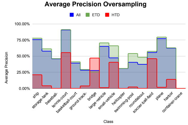
(b) Average precision experiment 1. Here 5 classes were not detected for HTD instances. The best performance is on tennis-courts.
