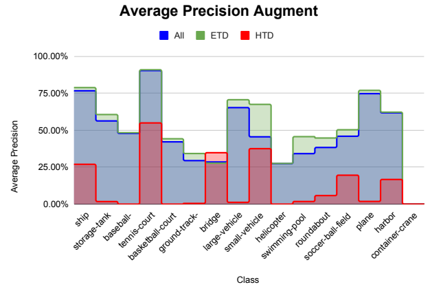
(c) Average precision experiment 2. Here 4 classes were not detected for HTD instances. The best performance is on tennis-courts.
