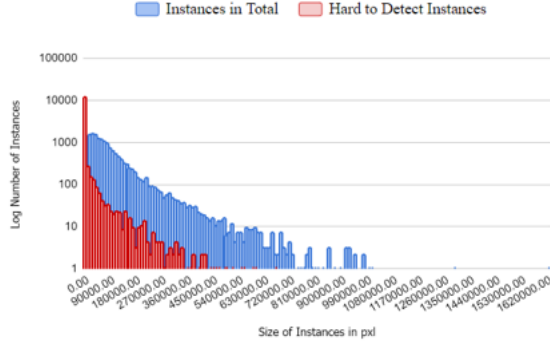
Fig. 1: Histogram of DOTA instances size. HTD instances tend to be smaller than the average instance.
