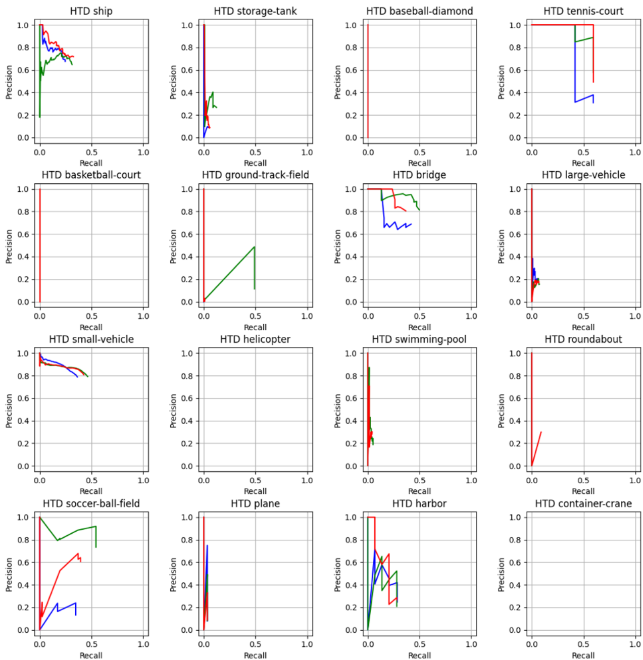
Fig. 5: Precision-Recall Curves for HTD instances. The blue line indicates the BL model, the green line the model from experiment 1 and the red line the model from experiment 2. The approach in experiment 1 improved the curves of the classes storage-tank, ground-track field, bridge, small-vehicle and soccer-ball-field. The approach from experiment 2 improved the performance on the classes ship, tennis-court, roundabout and harbor the most.
