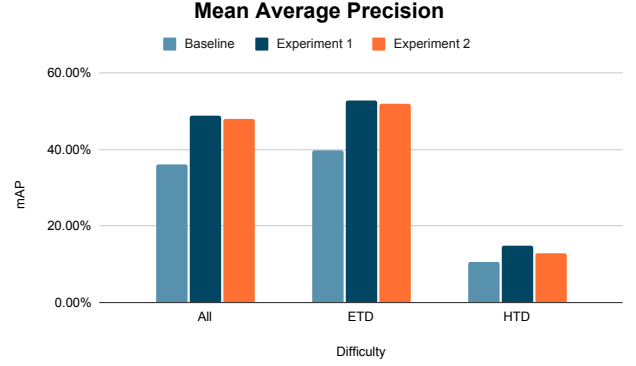
Fig. 3: Mean average precision. Both experiments improved the detection of instances in all difficulties. ETD instances have the highest mAP and HTD the lowest mAP. However, the approach in experiment 1 has a slightly better performance than the one in experiment 2.
