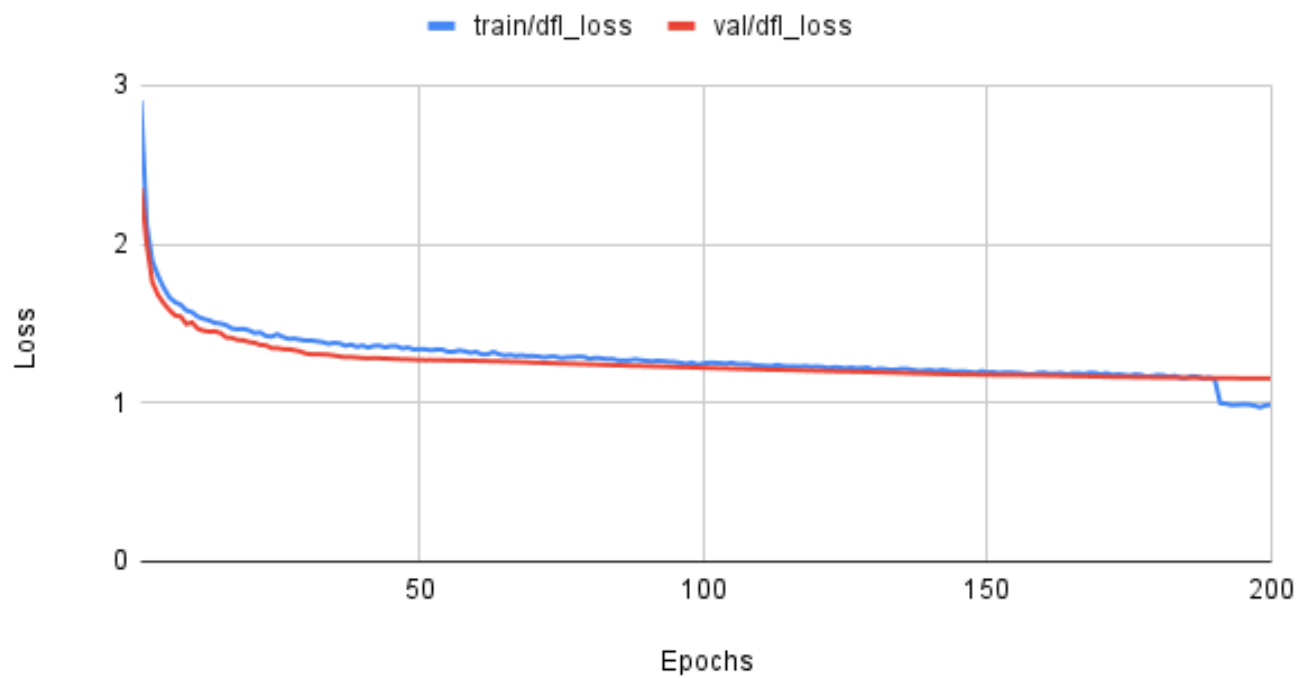
Fig. 18: Distribution Focal Loss on the Baseline model. The blue line indicates the training loss and the red line indicates the loss of the validation data.
