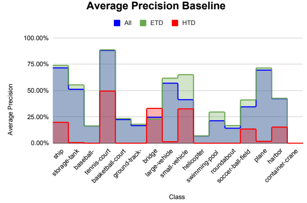
(a) Average precision BL. Here 7 classes were not detected for HTD instances. The best performance is on tennis-courts.
