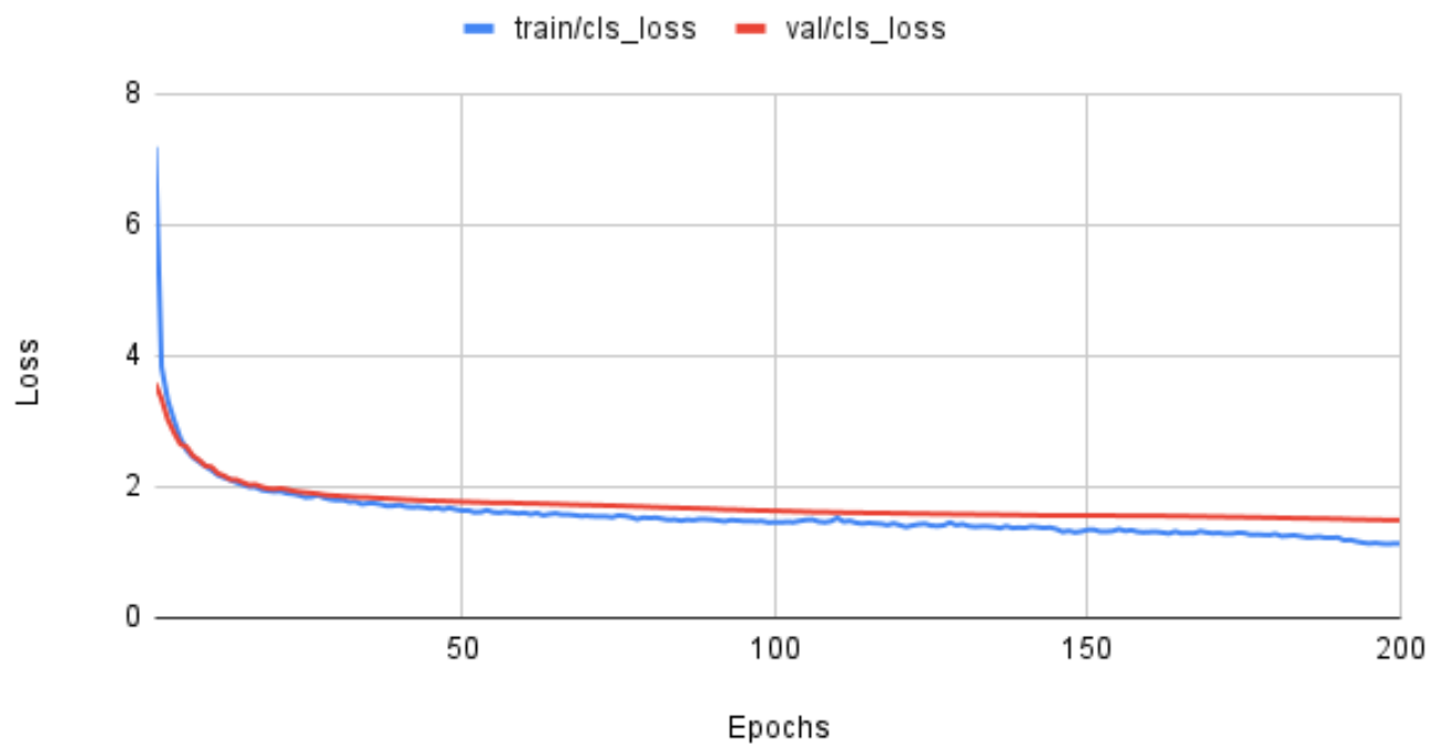
Fig. 20: Classification Loss on the Experiment 1 model. The blue line indicates the training loss and the red line indicates the loss of the validation data.
