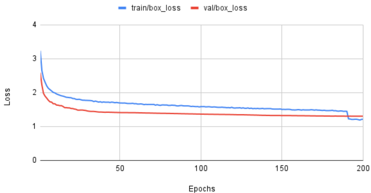
Fig. 16: Bounding box Loss on the Baseline model. The blue line indicates the training loss and the red line indicates the loss of the validation data.
