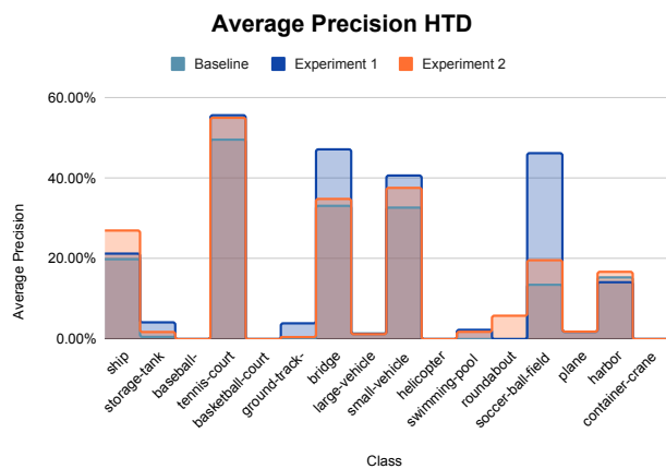
Fig. 10: Average precision of HTD instances. Comparing the AP across all three models it is evident that both approaches in experiment 1 and 2 improved the detection of HTD instances. The model from experiment 2 detected one class more (roundabout) than the model from experiment 1, however the latter model shows higher AP in many classes.
