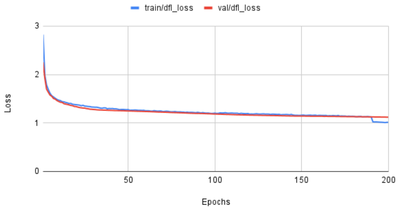
Fig. 21: Distribution Focal Loss on the Experiment 1 model. The blue line indicates the training loss and the red line indicates the loss of the validation data.
