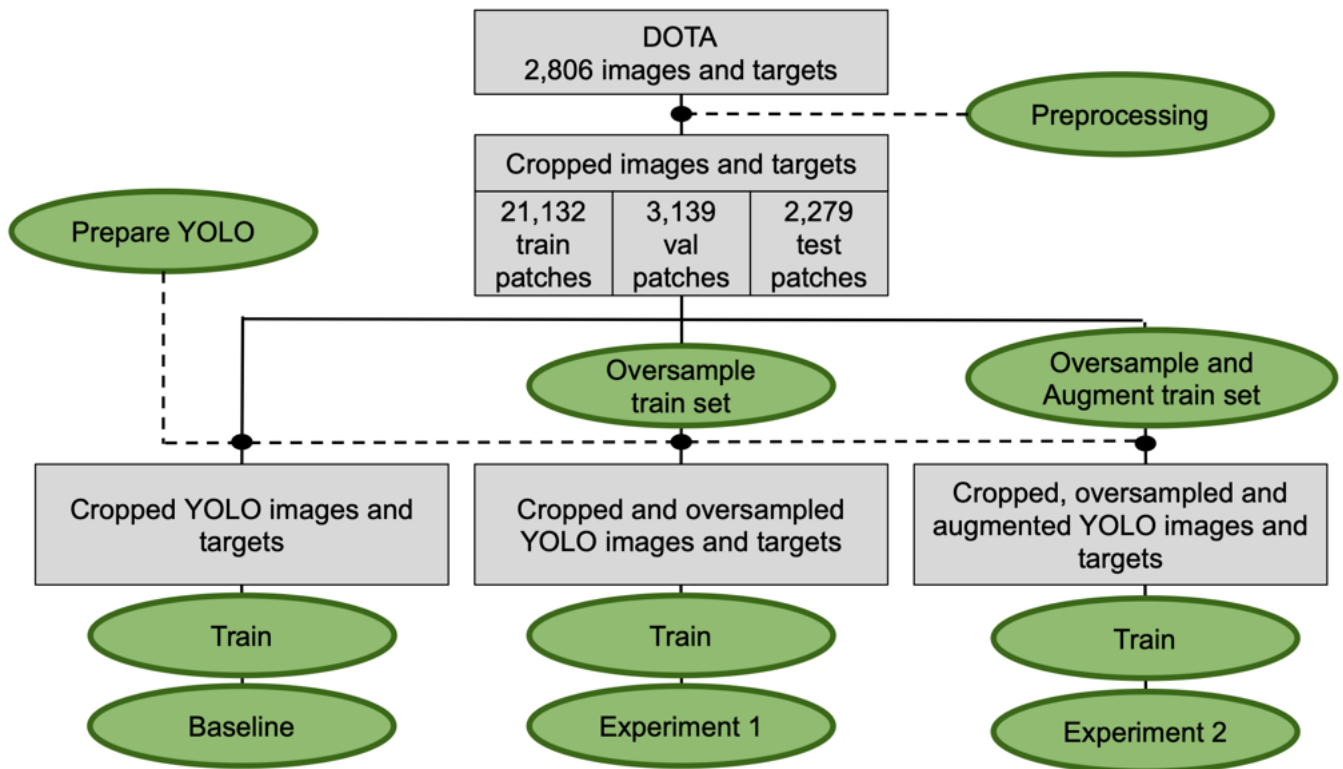
Fig. 4: Flowchart of the methodology. The images are split into patches of uniform size during preprocessing and are then handled in different ways according to the respective experiment.
