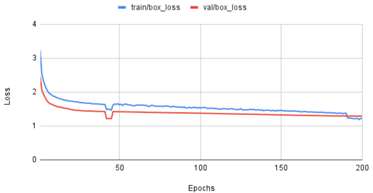
Fig. 22: Bounding Box Loss on the Experiment 2 model. The blue line indicates the training loss and the red line indicates the loss of the validation data.
