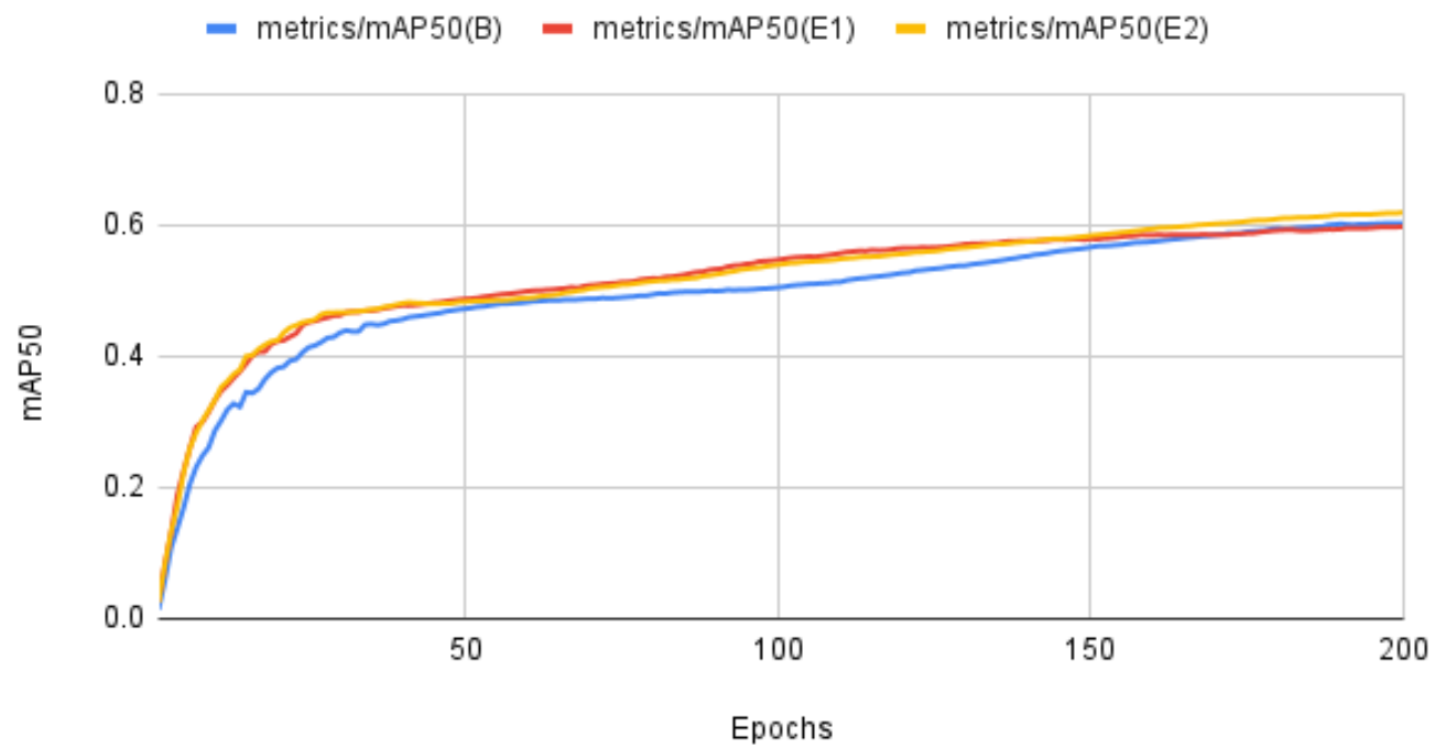
Fig. 25: Mean Average Precision of all three models. The blue line indicates the baseline, the red line indicates the first experiment and the yellow line represents the second experiment.
