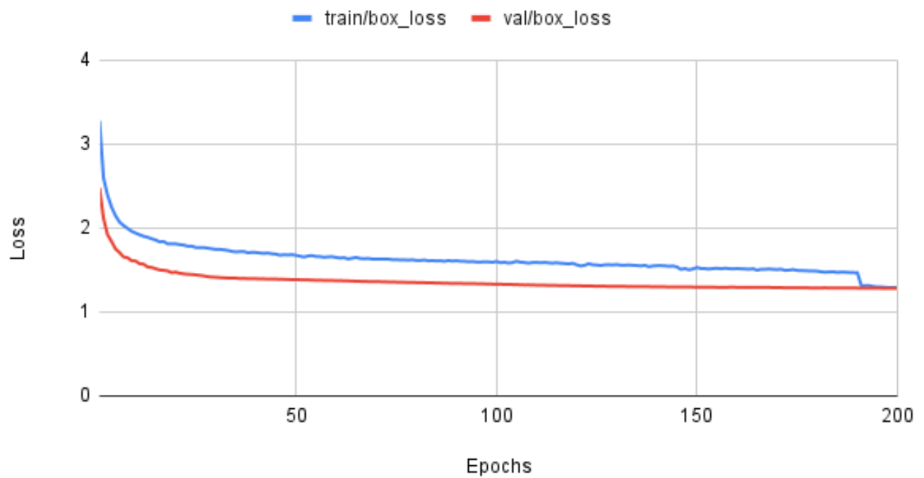
Fig. 19: Bounding Box Loss on the Experiment 1 model. The blue line indicates the training loss and the red line indicates the loss of the validation data.
